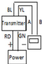
Figure 2 RS485 output
