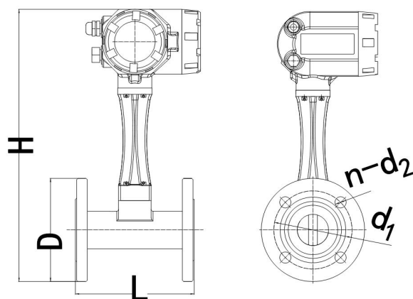
Flange connection fig. 2
