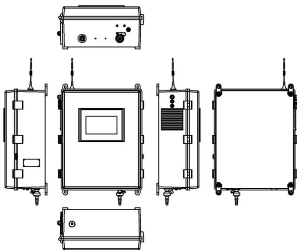
Fig.4 View of the equipment in all directions
