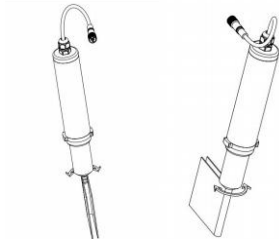
Fig.13 Polishing of Membraneless Dual Platinum Ring sensor
