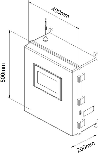
Fig.1 Product dimensions
